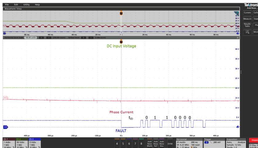
Figure 33 – 240 to 200 V_{DC} , Slew Rate: 5 V / ms.
