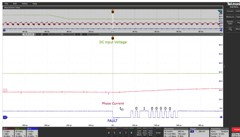
Figure 32 – 325 to 240 V_{DC} , Slew Rate: 5 V / ms.
