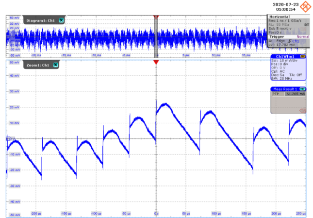
Figure 80 – Output Voltage Ripple Waveforms. 230 VAC, 137.5 mA Output. 10 mV, 5 ms / div.; 50 μs / div. V_{PK-PK} : 61.3 mV.
