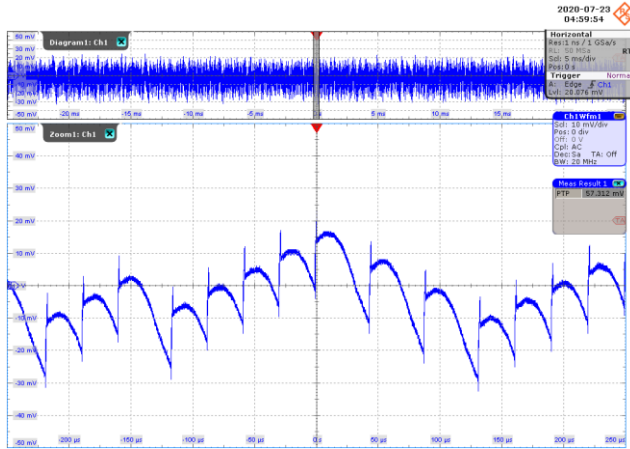
Figure 79 – Output Voltage Ripple Waveforms. 230 VAC, 275 mA Output. 10 mV, 5 ms / div.; 50 μs / div. V_{PK-PK} : 57.3 mV.
