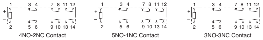
RF1V (6-pole)
