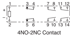
RF1V (6-pole)
