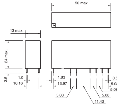
RF1V (6-pole)
