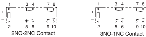
RF1V (4-pole)
