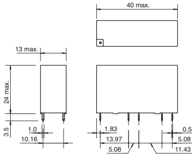
RF1V (4-pole)
