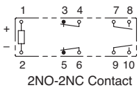
RF1V (4-pole)
