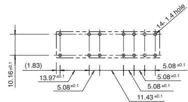
RF1V (6-pole)
