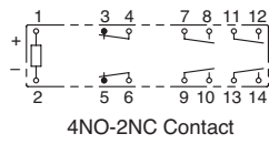
RF1V (6-pole)
