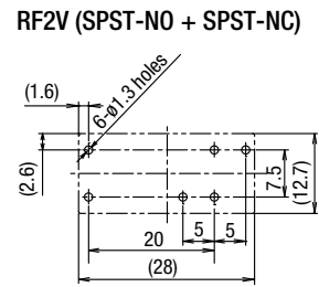
PC Board Terminal Mounting Hole Layout (Bottom View)
