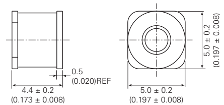
Surface-mount (GTCS25-XXXM-R02)
