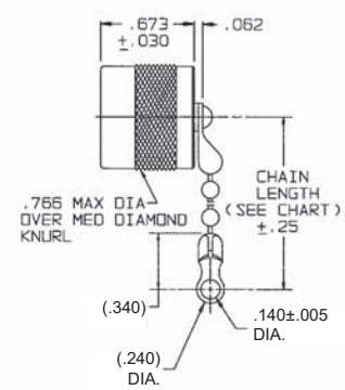
RFI85/RFI853-2 THRU -11 SHOWN STANDARD CHAIN & MOUNTING LUG
