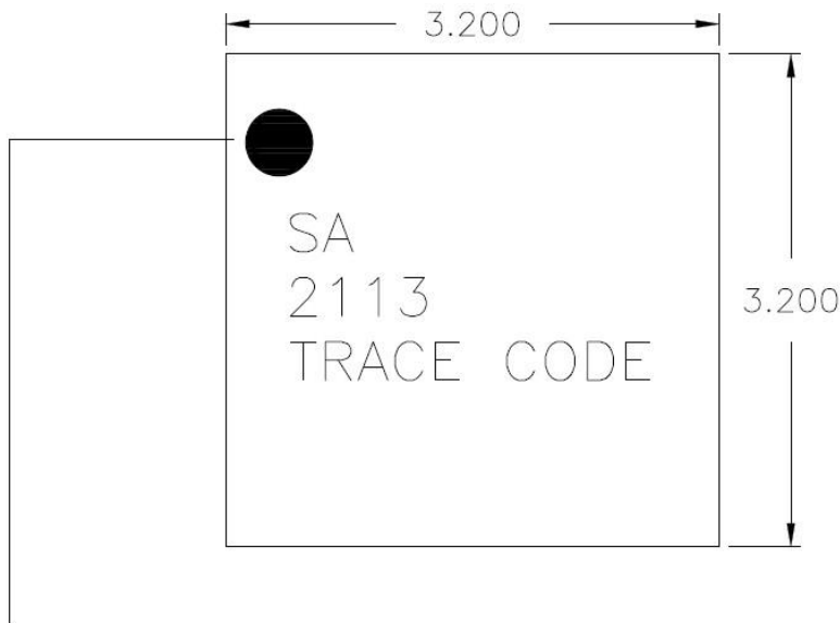
Pin 1 Indicator
