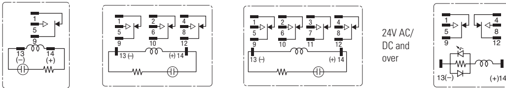
DPDT
