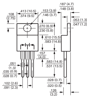
TO-220
