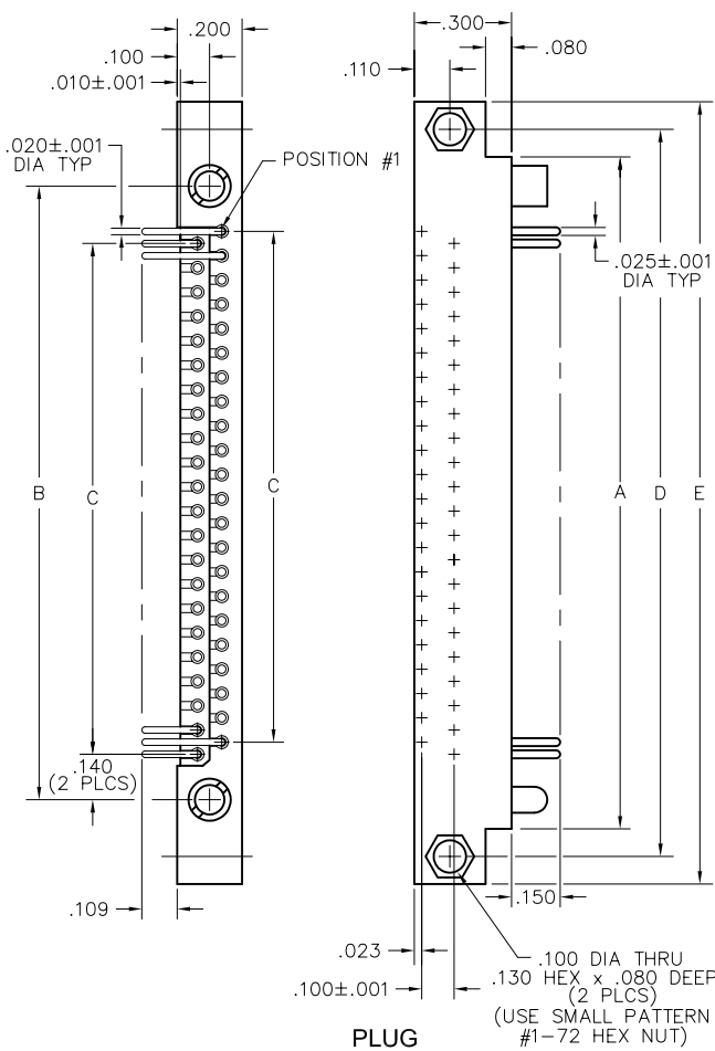
PLUG
