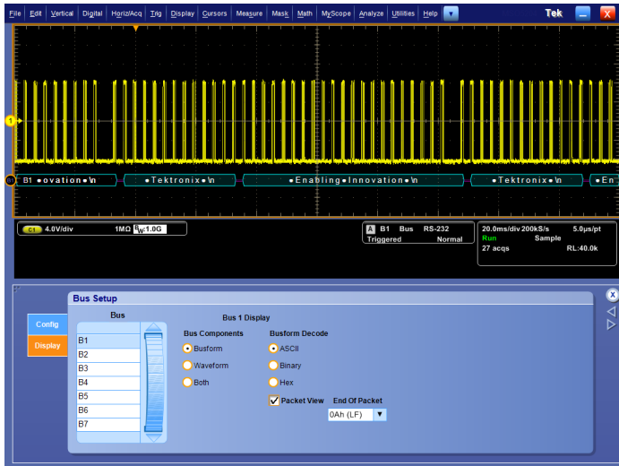
Packet View display of decoded RS-232 messages.
