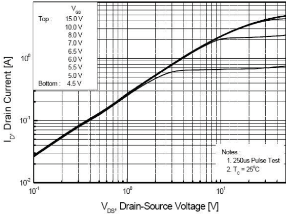
Fig. 1 On-State Characteristics
