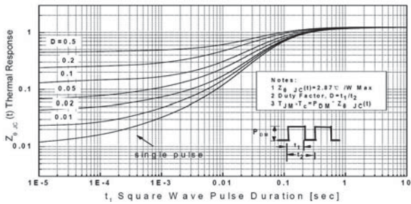
Fig. 9 Transient Thermal Response Curve (TO-251/TO-252)
