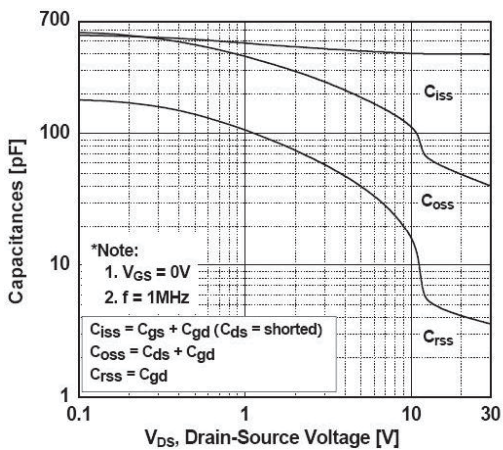
Fig. 5 Capacitance Characteristics
