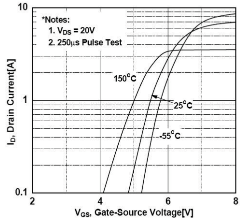
Fig. 2 Transfer Characteristics
