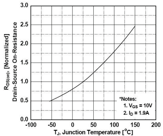
Fig. 4 On-Resistance Variation vs Temperature
