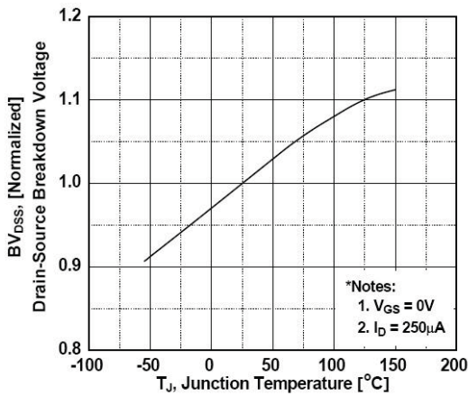
Fig. 3 Breakdown Voltage Variation vs Temperature
