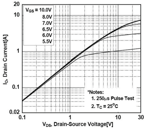
Fig. 1 On-State Characteristics
