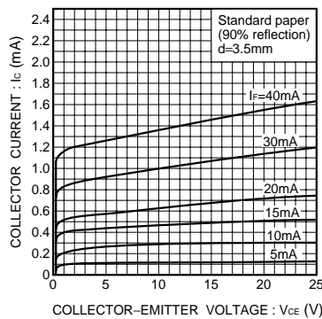
Fig.5 Output characteristics
