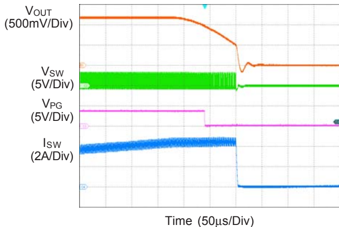
Figure 2. Over-Current Protection
