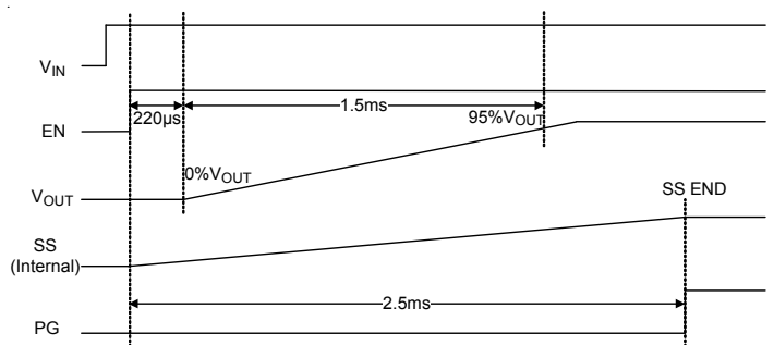
Figure 1. Start-Up Sequence
