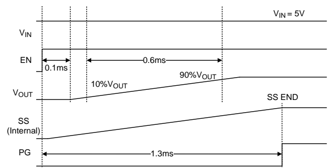
Figure 1. Start-Up Sequence
