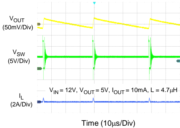
Output Ripple as IOUT = 10mA
