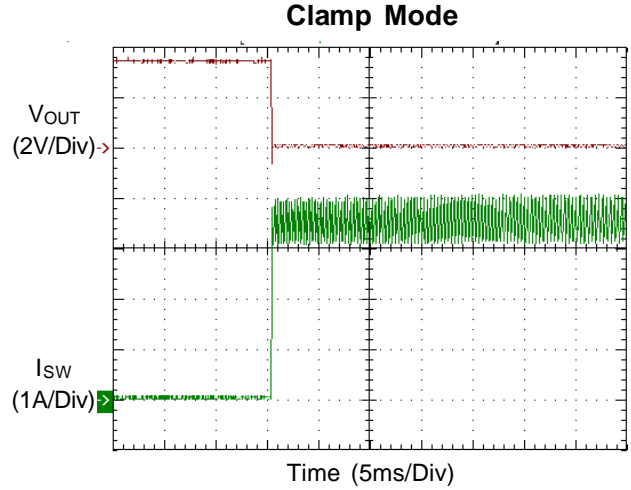
Figure 7. Clamp Mode
