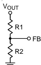
Figure 4. Setting V OUT with a Resistive Voltage Divider
