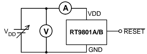
Current Consumption
