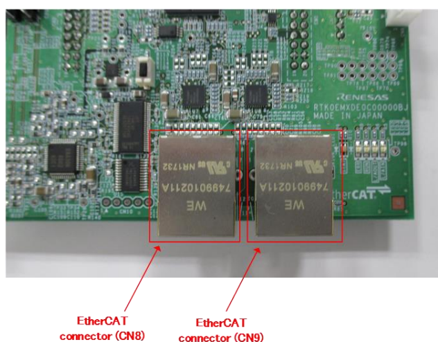
Figure 5-2 EtherCAT Connector
