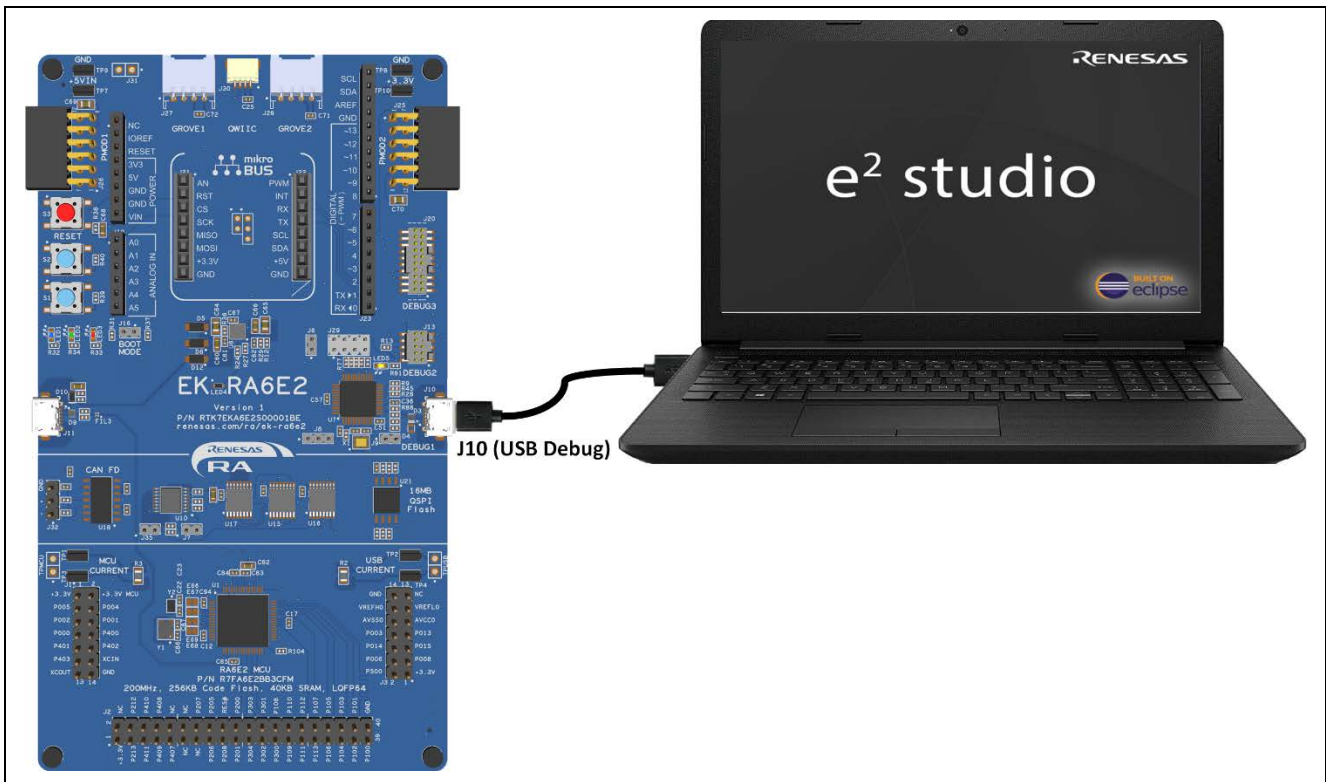
Figure 23. Connecting the EK-RA6E2 Board to the Host PC via USB Debug Port
