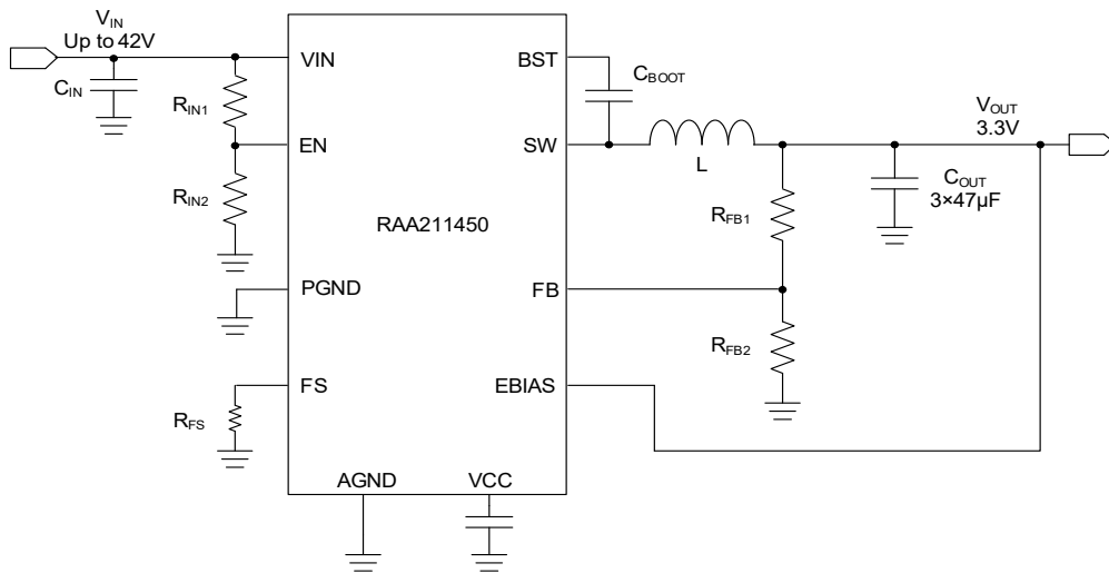
Figure 1. Simplified Circuit
