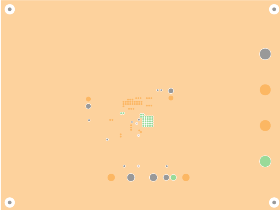
Figure 6. Second Layer
