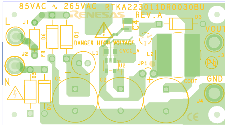
Figure 5. Top Layer
