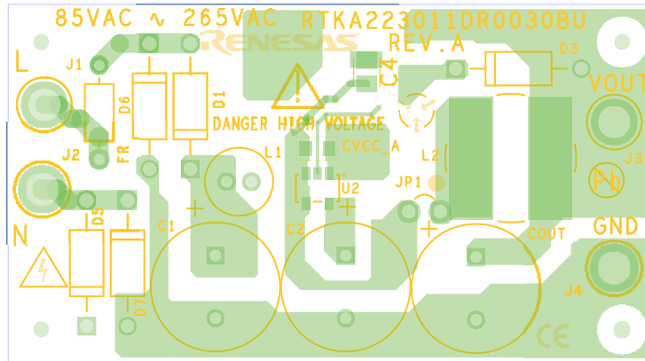
Figure 5. Top Layer [1]
