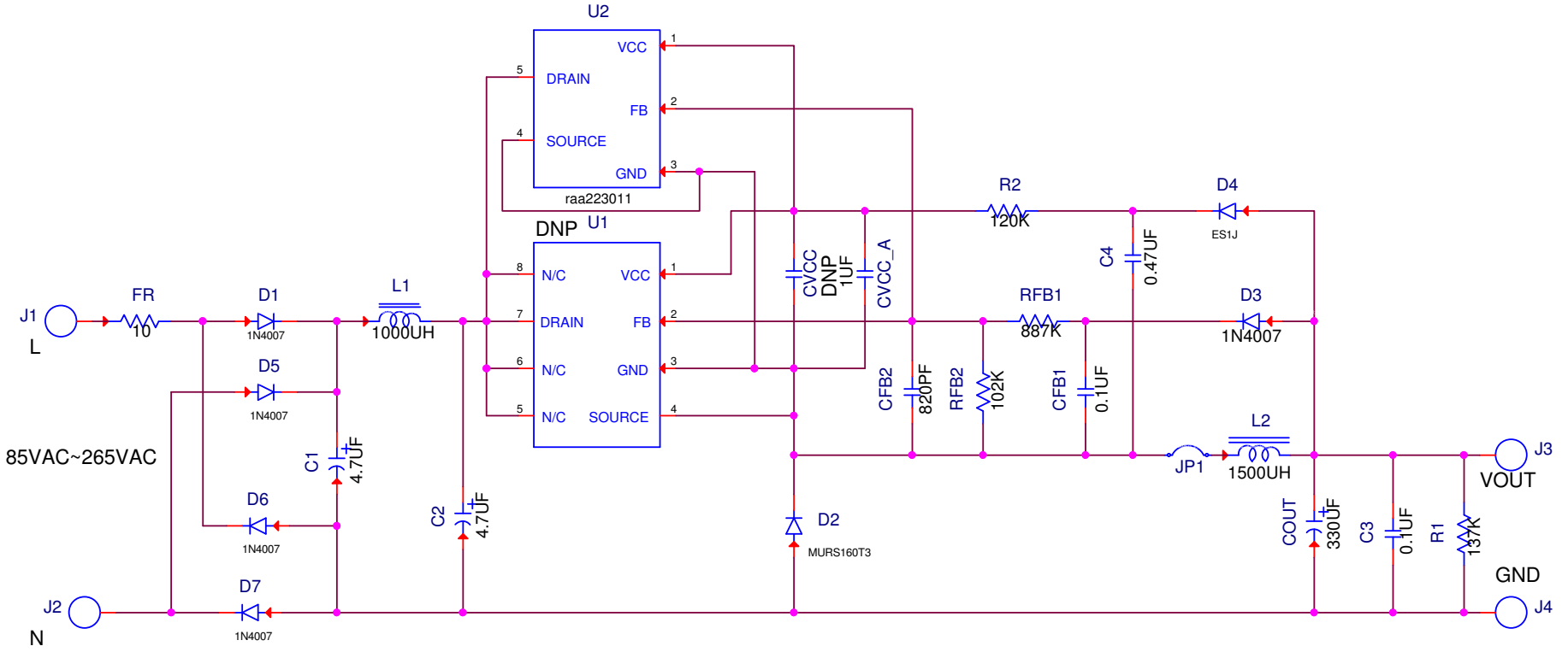
Figure 4. RTKA223011DR0040BU Schematic
