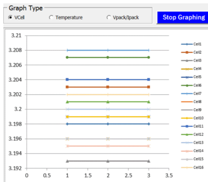
Figure 66. VCell Graph
