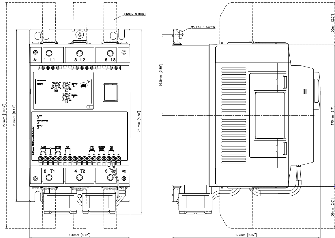
Fig. 4 RSWT 120 mm (70 Arms - 90 Arms)
