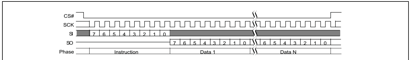
Figure 117 Password read (PASSRD E7h) command sequence
