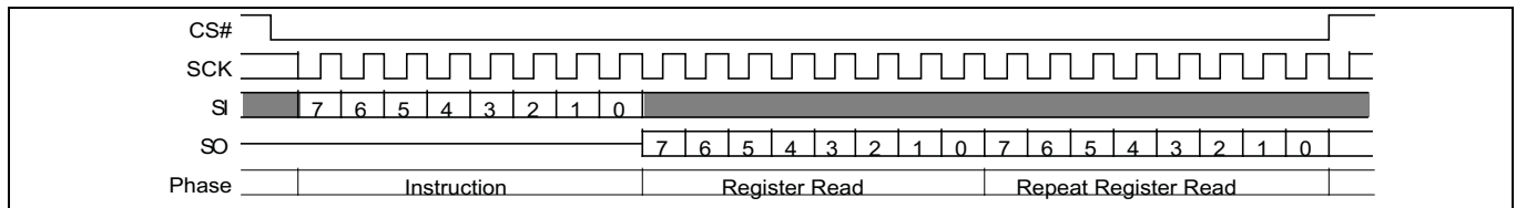
Figure 108 ASPRD command
