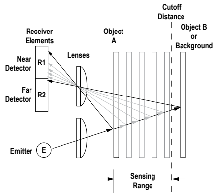
Object is sensed if amount of light at R1 is greater than the amount of light at R2 Figure 1. Fixed-Field Concept
