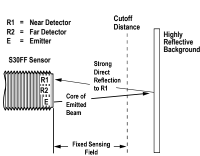
Figure 3. Reflective Background - Problem
