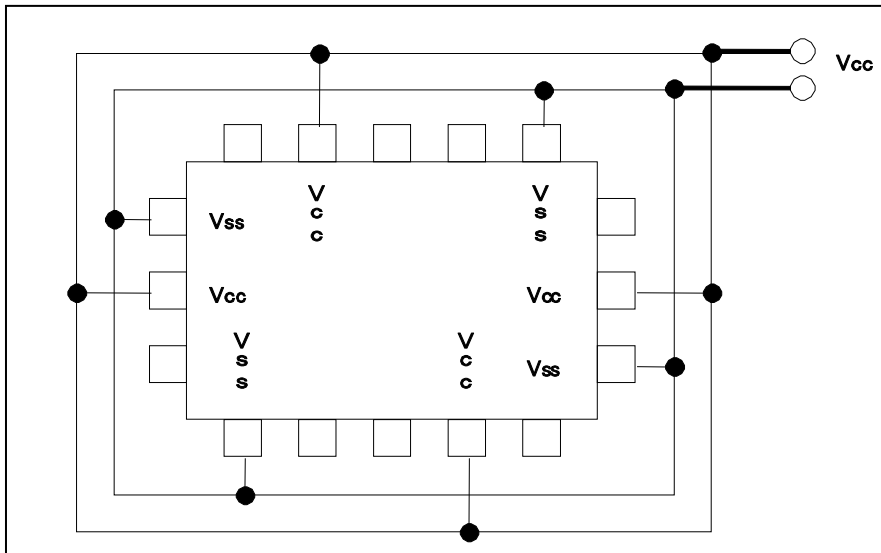
Figure 8-1 Pin Assignment
