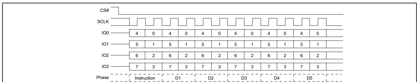
Figure 42 Read Identification (RDID) QPI mode command
