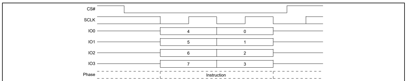
Figure 105 DPD command sequence QPI mode
