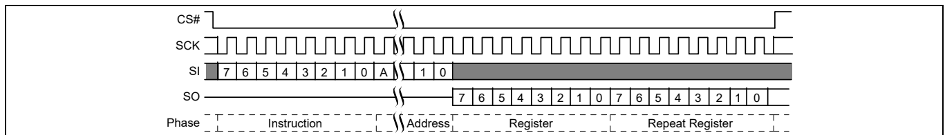
Figure 89 DYBRD command sequence [57, 58]
