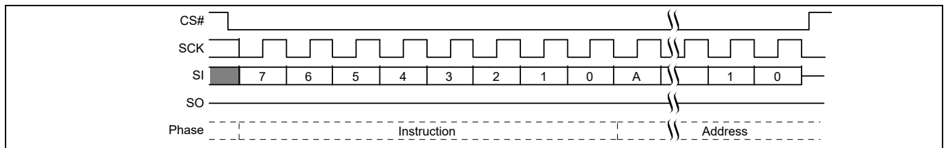
Figure 81 EES command sequence [56]
