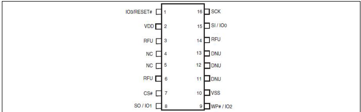
Figure 36 16-lead SOIC package, Top view [34]
