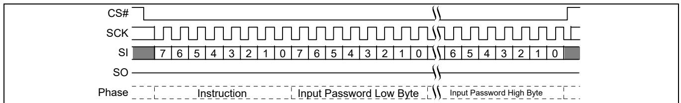
Figure 99 Password Unlock command sequence
