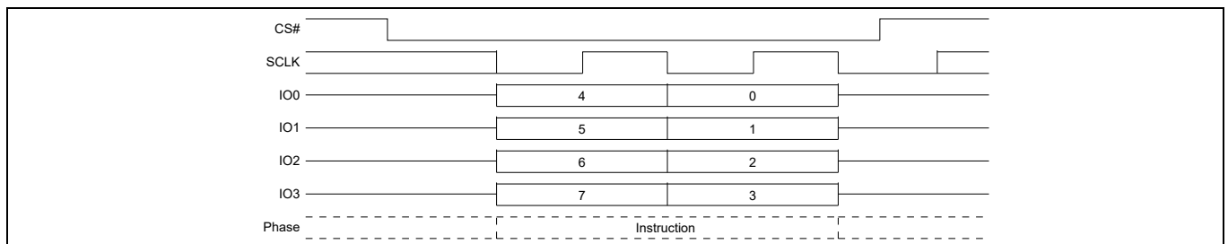
Figure 103 Mode Bit Reset command sequence QPI mode
