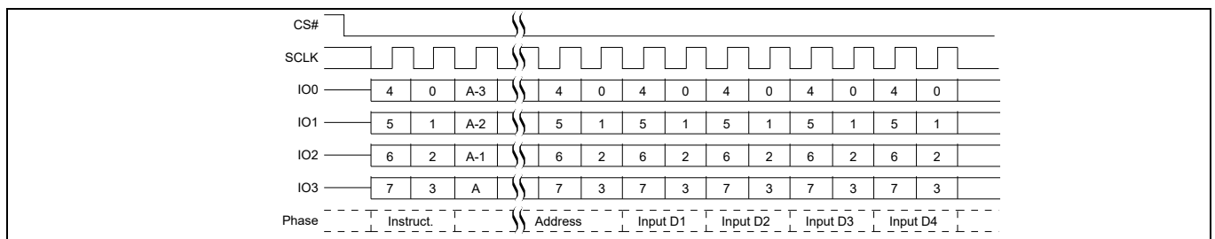
Figure 74 Page Program (PP 02h or 4PP 12h) QPI mode command sequence [52]
