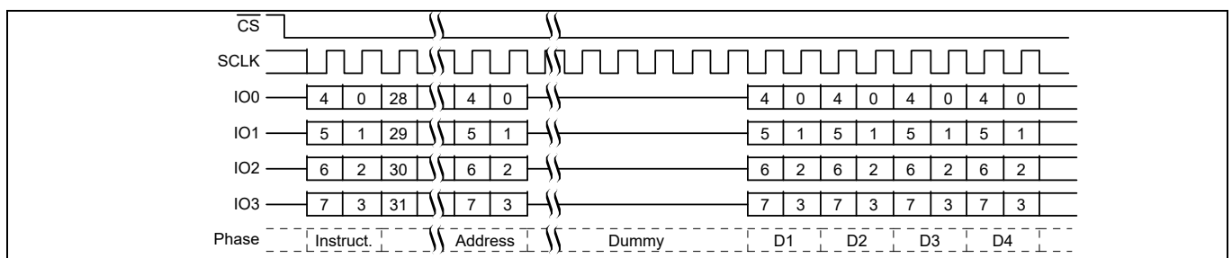
Figure 54 ECCRD (19h), Quad All Mode, CR2[7] = 1, or 4EECRD (18h) command sequence
