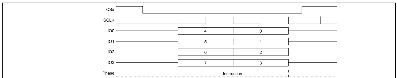
Figure 47 Write Enable (WREN) command sequence QPI mode
