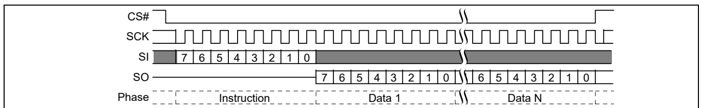
Figure 41 Read Identification (RDID) command sequence
