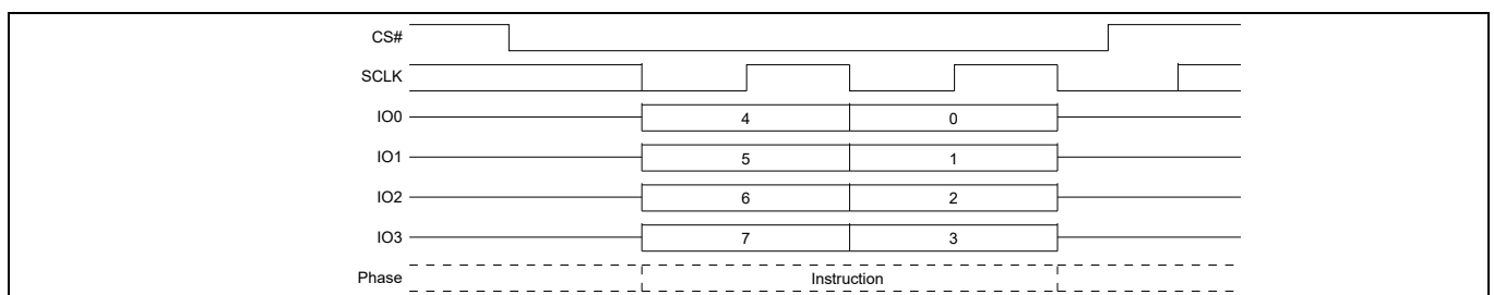
Figure 85 Erase or Program Suspend command sequence QPI mode
