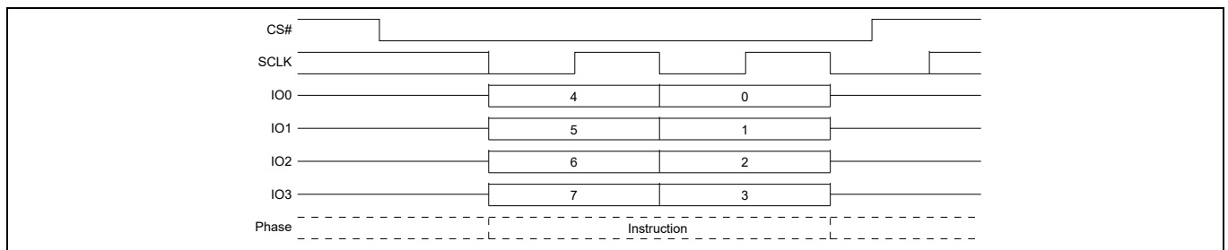
Figure 107 RES command sequence QPI mode
