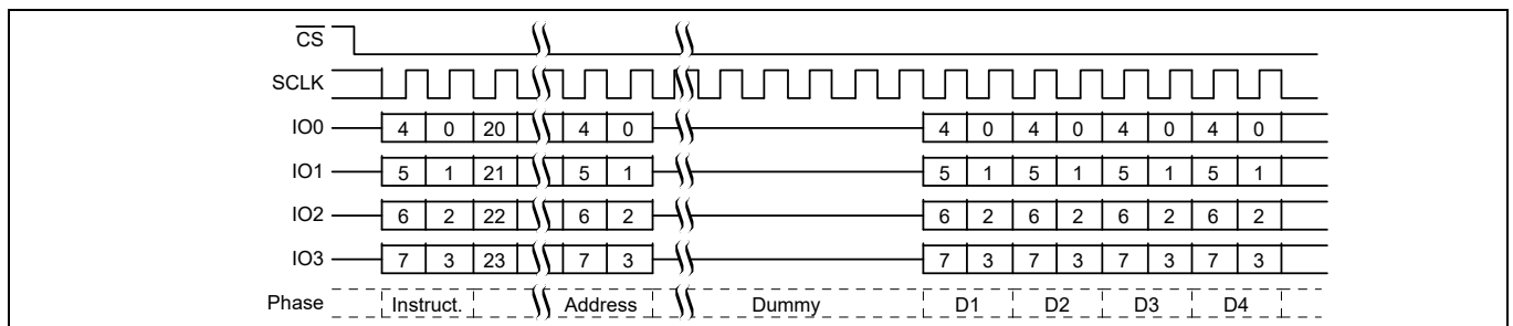
Figure 53 ECCRD (19h), Quad All Mode, CR2[7] = 0, command sequence
