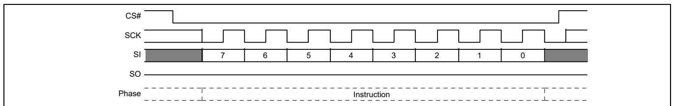
Figure 46 Write Enable (WREN) command sequence
