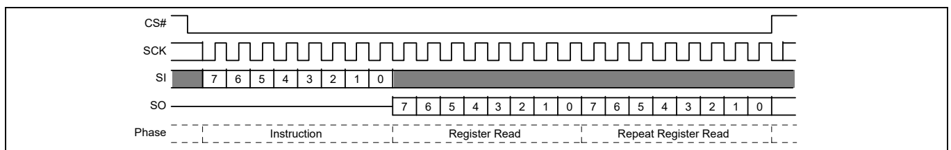
Figure 96 PPB Lock Register Read command sequence
