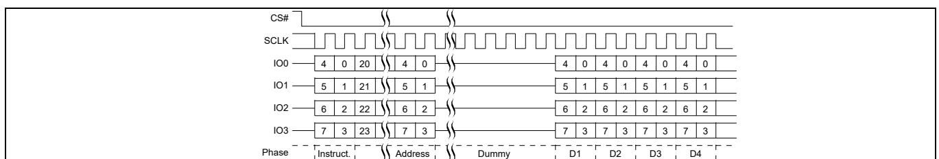
Figure 45 RSFDP QPI mode command sequence
