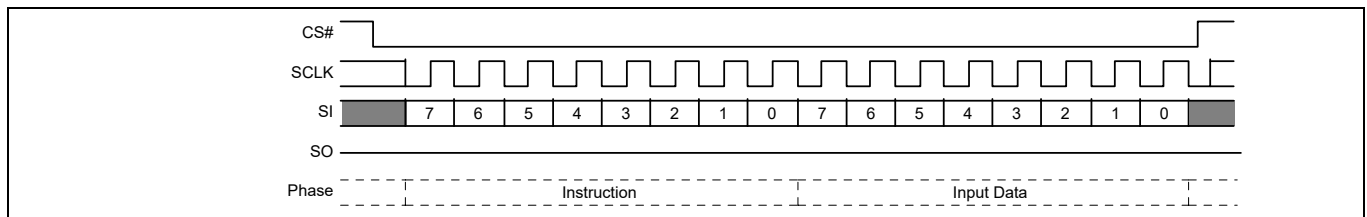
Figure 61 Set Burst Length command sequence
