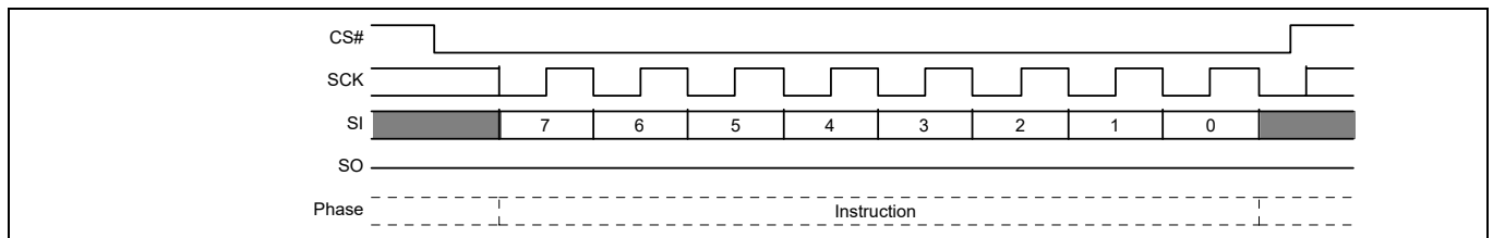
Figure 84 Erase or Program Suspend command sequence
