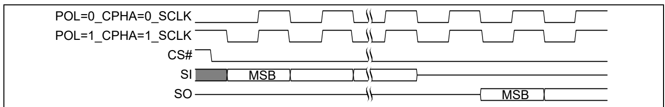
Figure 4 SPI SDR modes supported
