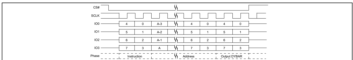
Figure 90 DYBRD QPI mode command sequence [57, 58]
