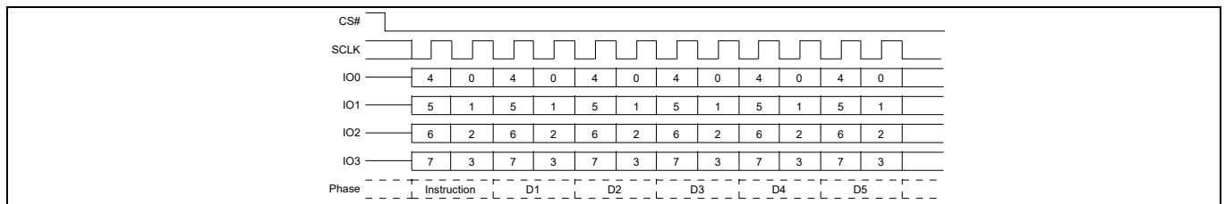
Figure 43 Read Quad Identification (RDQID) command sequence
