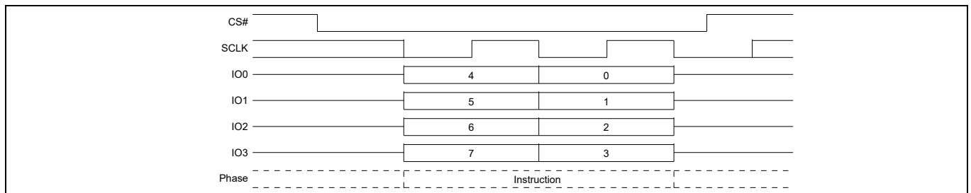
Figure 51 Clear Status Register (CLSR) command sequence QPI mode
