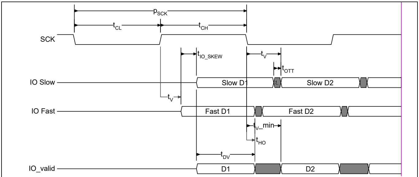
Figure 35 SPI DDR data valid window
