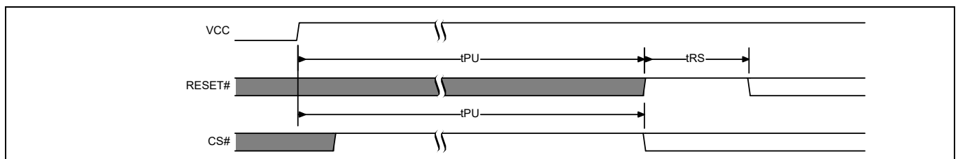
Figure 25 POR followed by hardware reset
