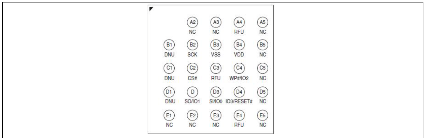
Figure 37 24-ball BGA, 5x5 ball footprint (FAB024), Top view [35, 36]
