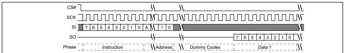
Figure 63 Fast Read (FAST_READ) command sequence (3-byte address, 0Bh [CR2V[7] = 0]) [47]
