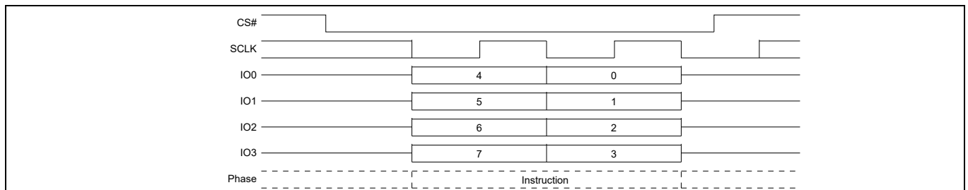
Figure 49 Write Disable (WRDI) command sequence QPI mode
