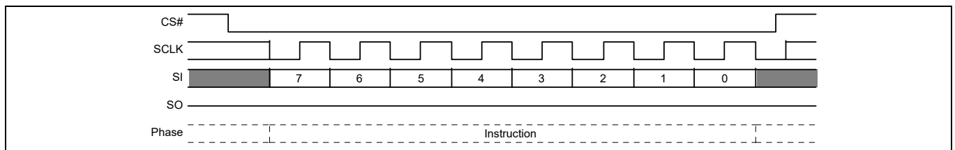
Figure 106 Release from Deep Power-down command sequence
