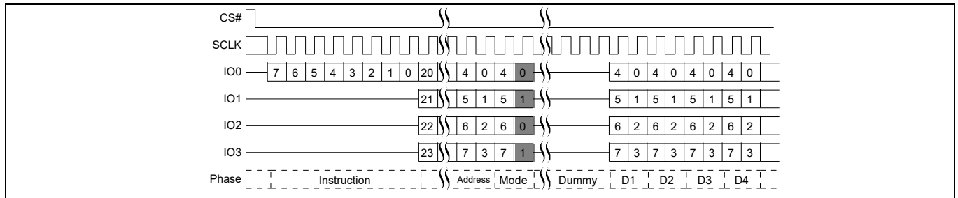
Figure 66 Quad I/O Read command sequence (3-byte address, EBh [CR2V[7] = 0])
