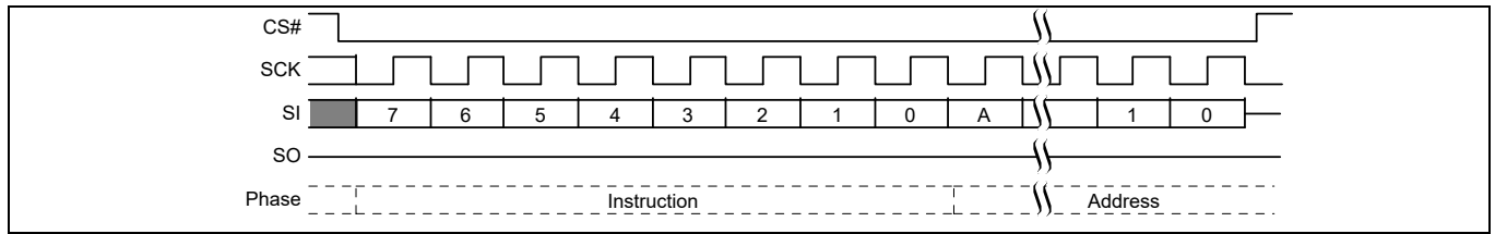
Figure 75 Parameter Sector Erase (P4E 20h or 4P4E 21h) command sequence [53]
