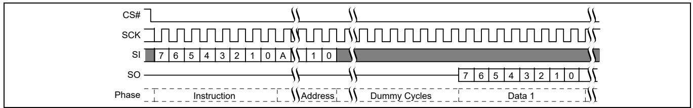
Figure 58 Read Any Register Read command sequence [45]
