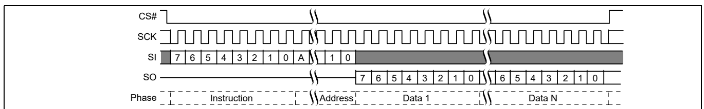
Figure 62 Read command sequence (3-byte address, 03h or 13h) [46]
