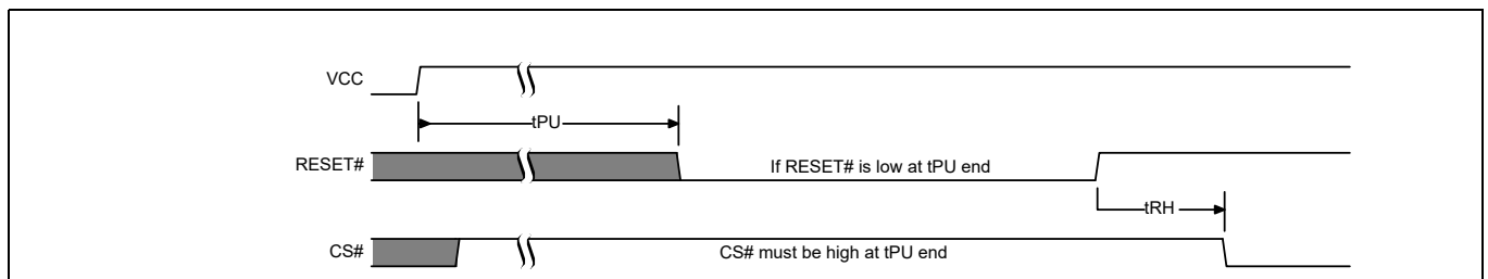
Figure 23 Reset LOW at the end of POR
