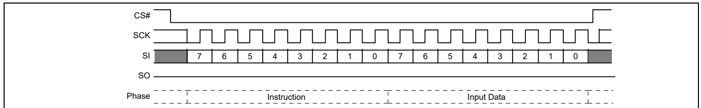
Figure 55 Write VDLR (WVDLR) command sequence
