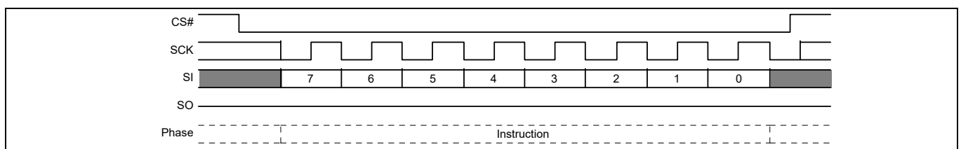
Figure 57 Enter 4 Byte Address Mode (4BAM B7h) command sequence
