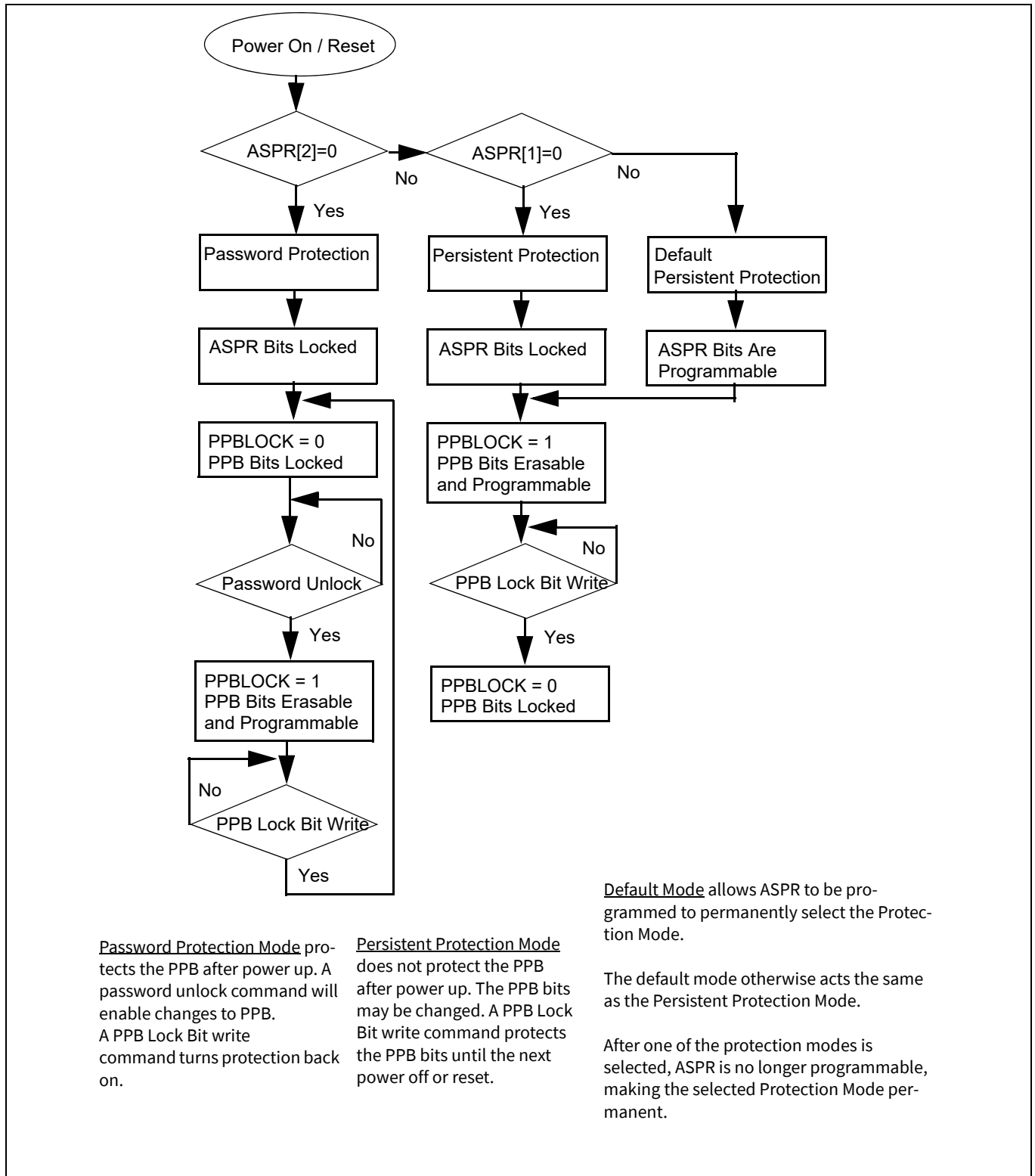
Figure 40 Advanced sector protection overview
