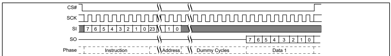
Figure 44 RSFDP command sequence
