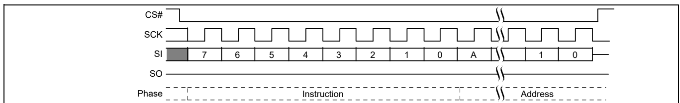
Figure 79 Bulk Erase Addressed command sequence [55]
