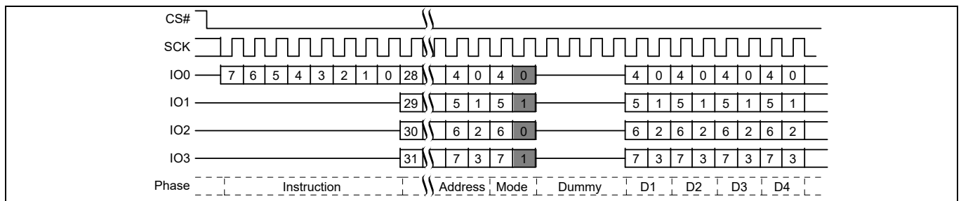
Figure 68 Quad I/O Read command sequence (4-byte address, ECh or EBh [CR2V[7] = 1])
