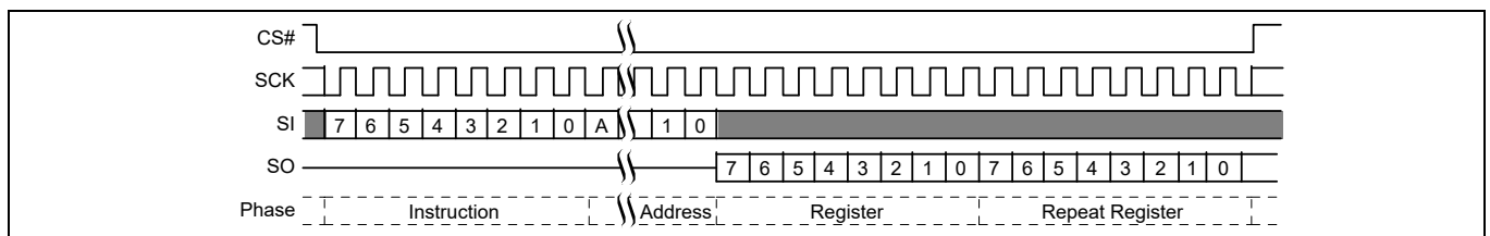
Figure 93 PPBRD command sequence [61, 62]
