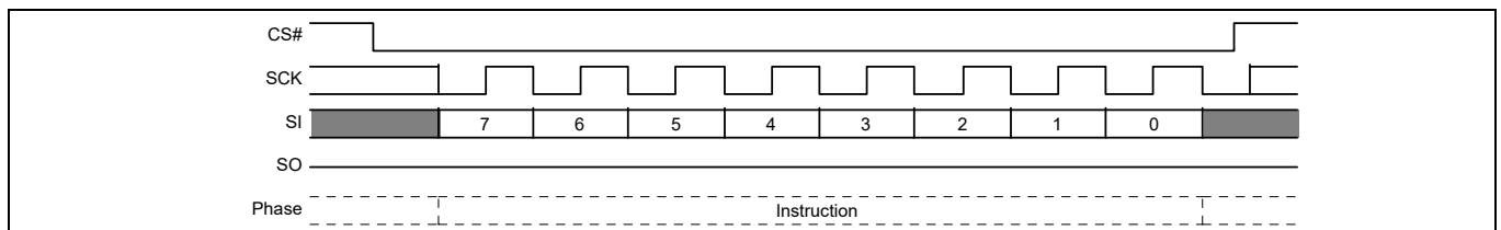
Figure 100 Software Reset command sequence
