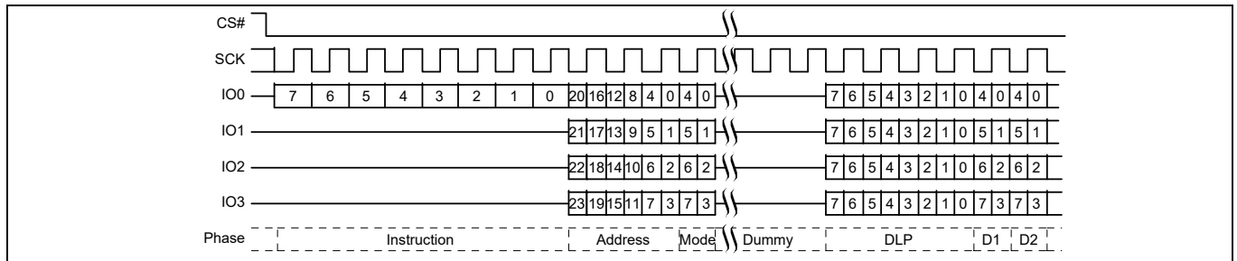
Figure 70 DDR Quad I/O Read initial access (3-byte address, EDh [CR2V[7] = 0])
