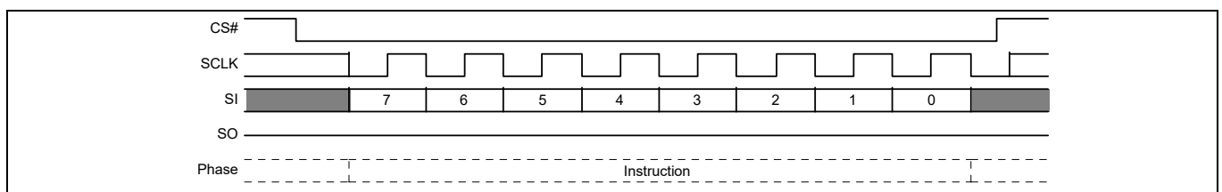
Figure 104 Deep Power-down command sequence
