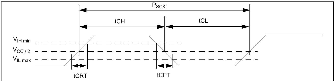
Figure 28 Clock timing
