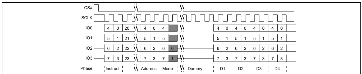
Figure 67 Quad I/O Read command sequence (3-byte address, EBh [CR2V[7] = 0]) QPI mode
