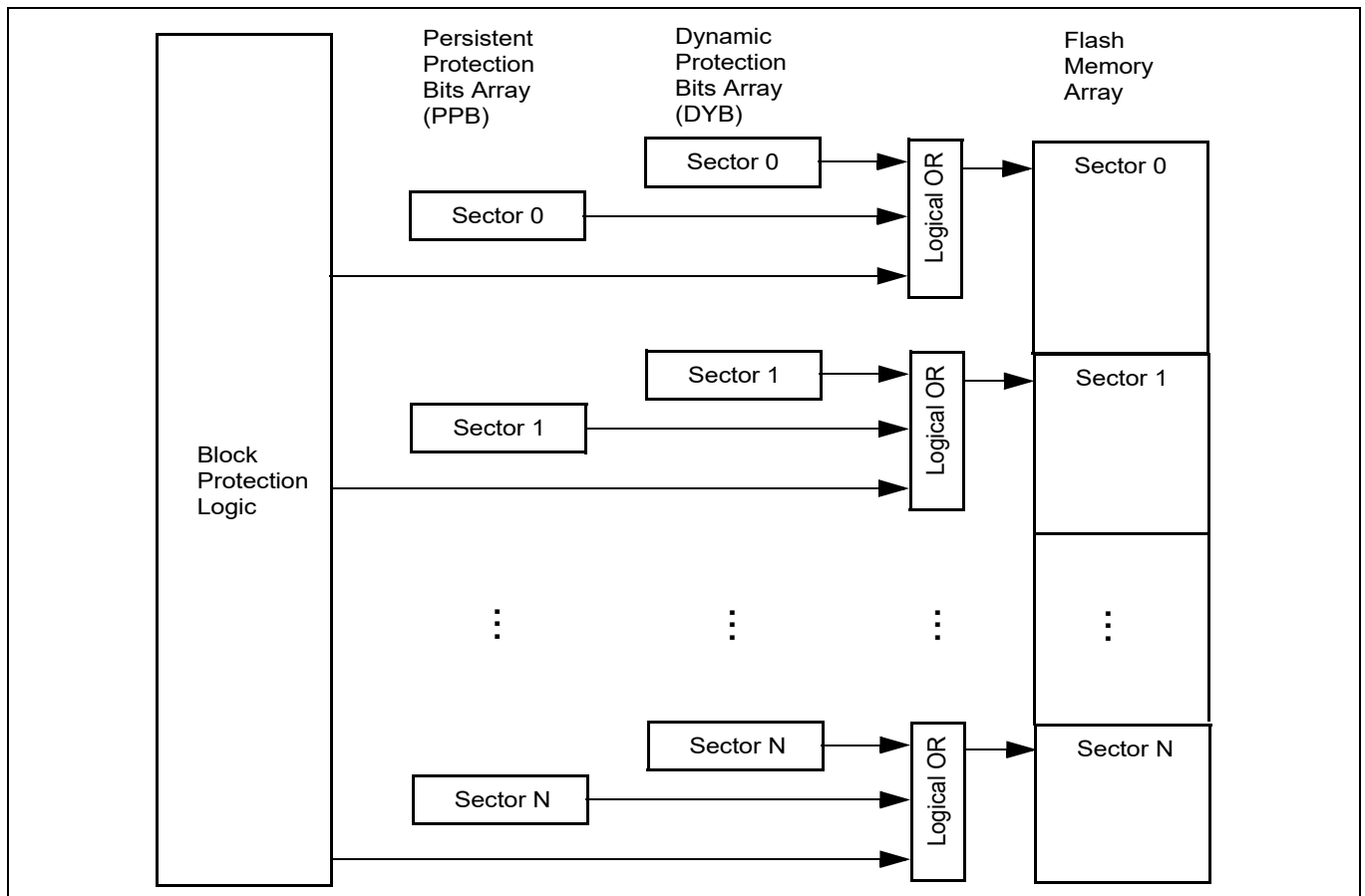
Figure 39 Sector protection control
