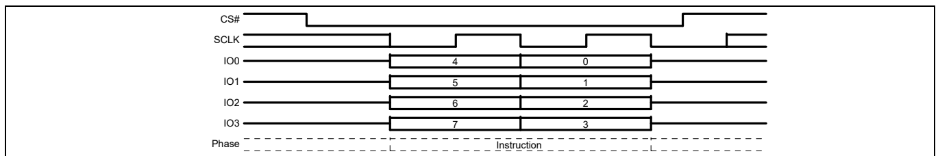
Figure 101 Software Reset command sequence QPI mode
