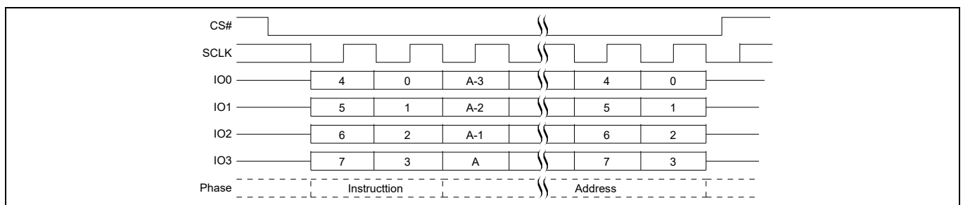
Figure 82 EES QPI mode command sequence [56]
