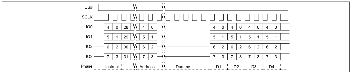
Figure 60 Read Any Register, QPI Mode, CR2[7] = 1, command sequence
