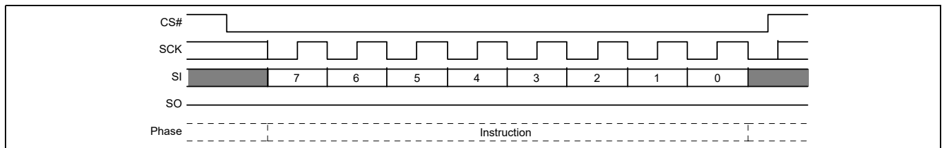
Figure 97 PPB Lock Bit Write command sequence
