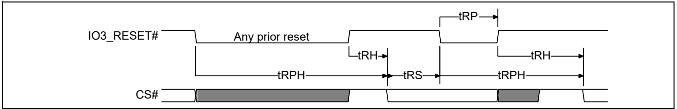
Figure 26 Hardware Reset when Quad mode is not enabled and IO3 / Reset# is enabled
