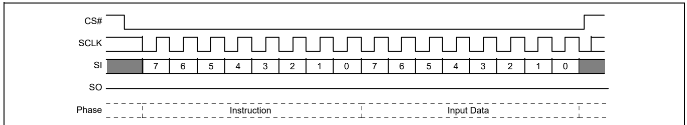
Figure 7 Single Bit Wide Input command
