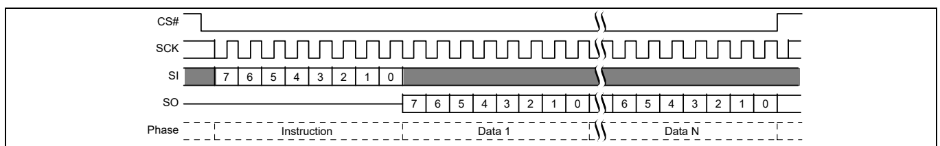
Figure 98 Password Read command sequence
