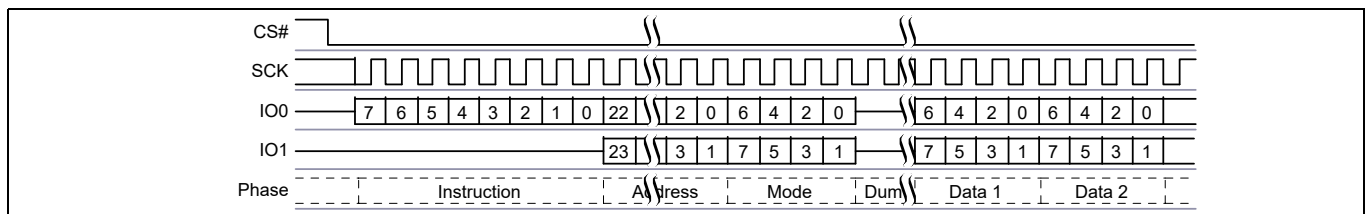
Figure 64 Dual I/O Read command sequence (3-byte address, BBh [CR2V[7] = 0]) [48]
