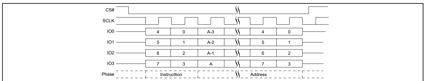
Figure 80 Bulk Erase Addressed command sequence QPI mode [55]
