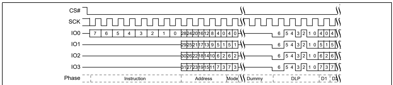
Figure 71 DDR Quad I/O Read initial access (4-byte address, EEh or EDh [CR2V[7] = 1]) [49]
