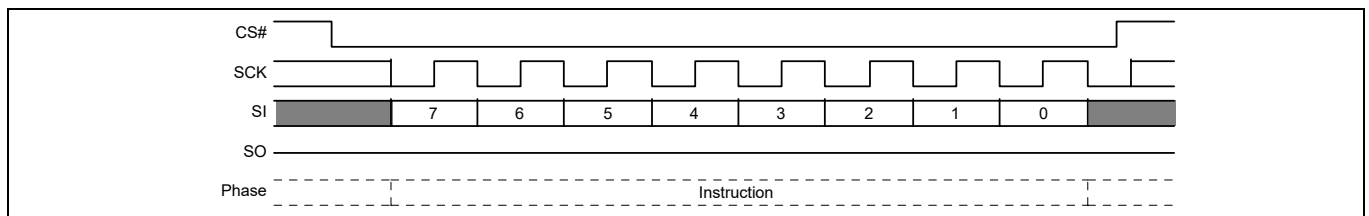
Figure 95 PPB Erase command sequence
