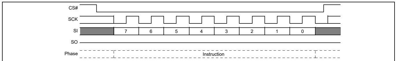
Figure 102 Mode Bit Reset command sequence
