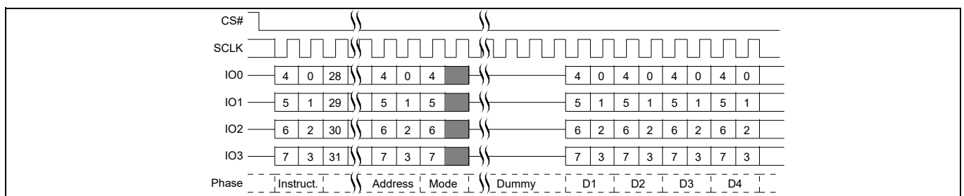
Figure 69 Quad I/O Read command sequence (4-byte address, ECh or EBh [CR2V[7] = 1]) QPI mode
