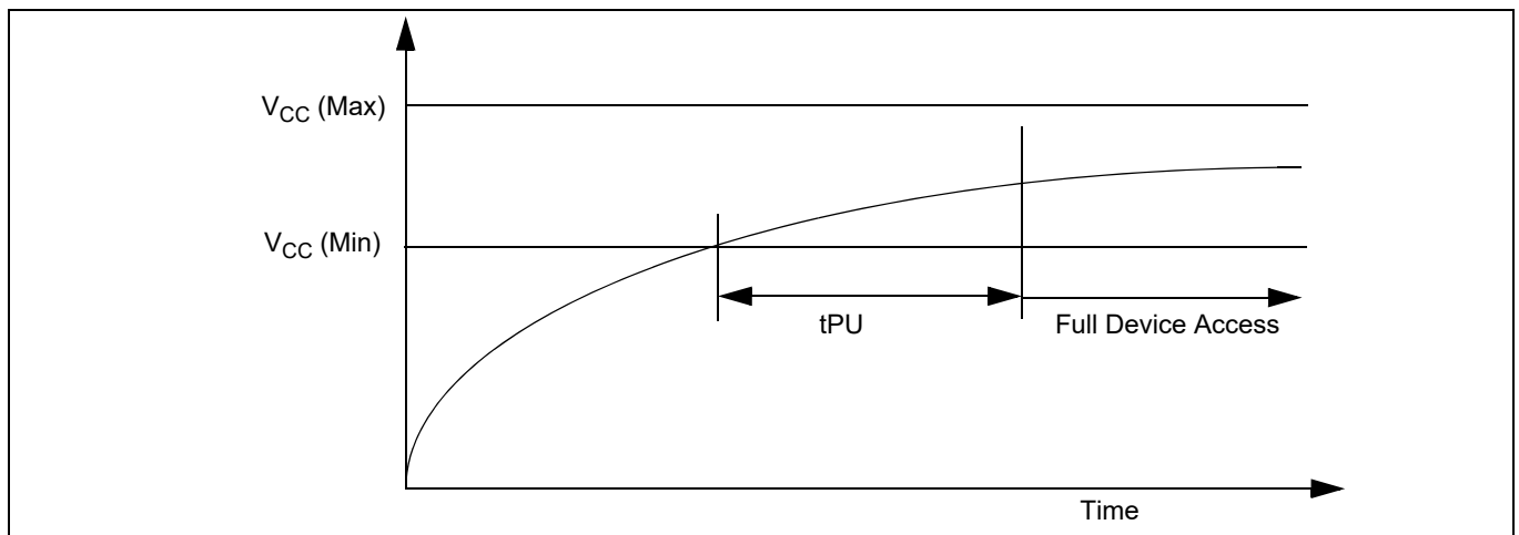
Figure 18 Power-up
