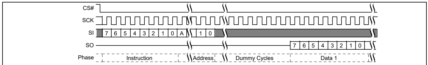
Figure 52 ECC Status Register Read command sequence [43, 44]
