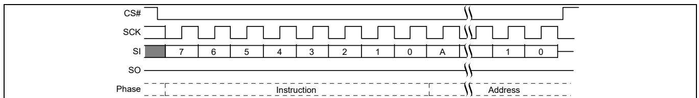
Figure 77 Sector Erase (SE D8h or 4SE DCh) command sequence [54]
