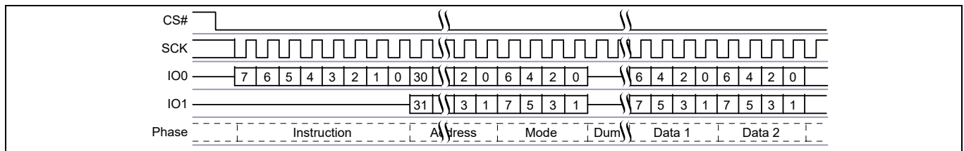
Figure 65 Dual I/O Read command sequence (4-byte address, BBh [CR2V[7] = 1])
