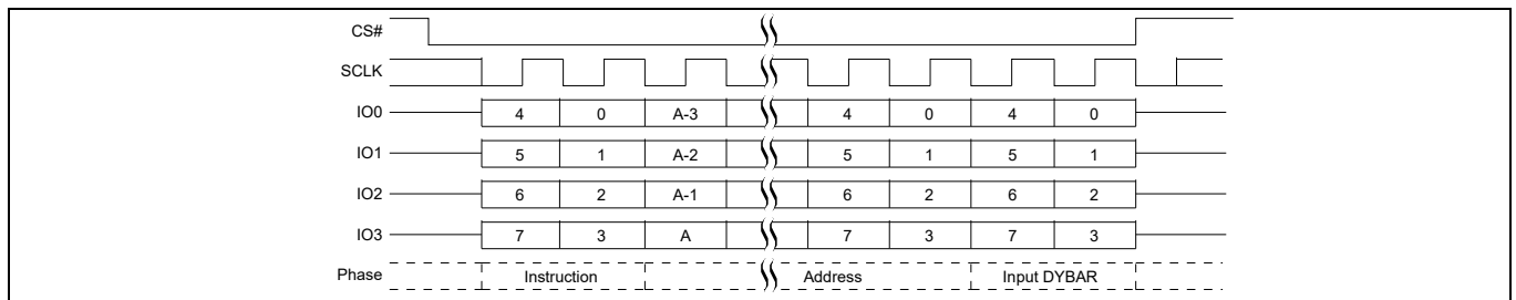
Figure 92 DYBWR QPI mode command sequence [59, 60]
