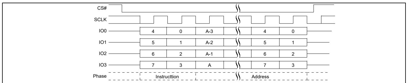
Figure 76 Parameter Sector Erase (P4E 20h or 4P4E 21h) QPI mode command sequence [53]
