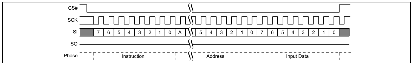
Figure 91 DYBWR command sequence [59, 60]
