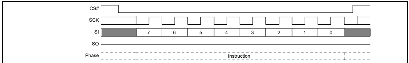
Figure 50 Clear Status Register (CLSR) command sequence
