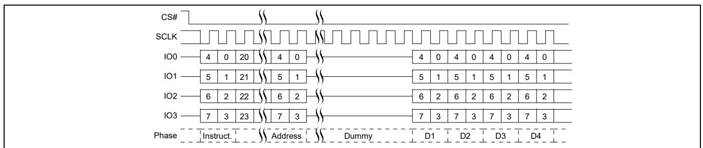
Figure 59 Read Any Register, QPI Mode, CR2[7] = 0, command sequence
