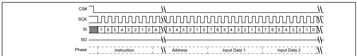
Figure 73 Page Program (PP 02h or 4PP 12h) command sequence [51]
