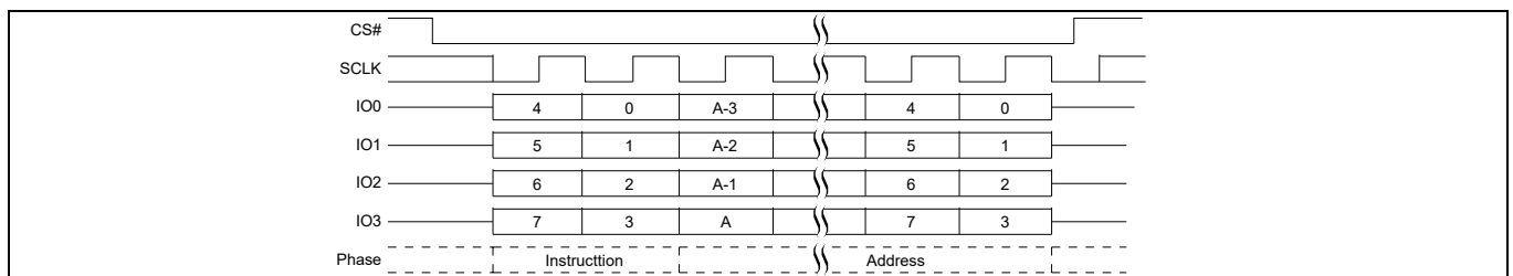
Figure 78 Sector Erase (SE D8h or 4SE DCh) QPI mode command sequence [54]
