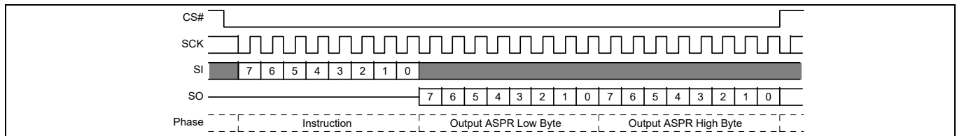
Figure 88 ASPRD command
