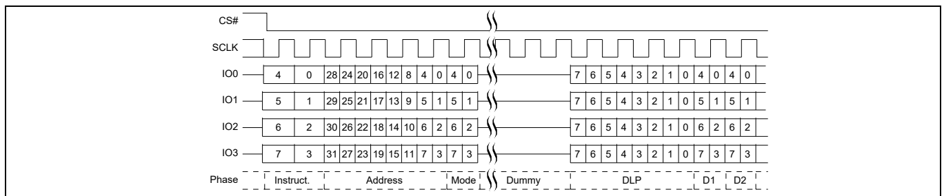
Figure 72 DDR Quad I/O Read initial access (4-byte address, EEh or EDh [CR2V[7] = 1]) QPI mode [50]
