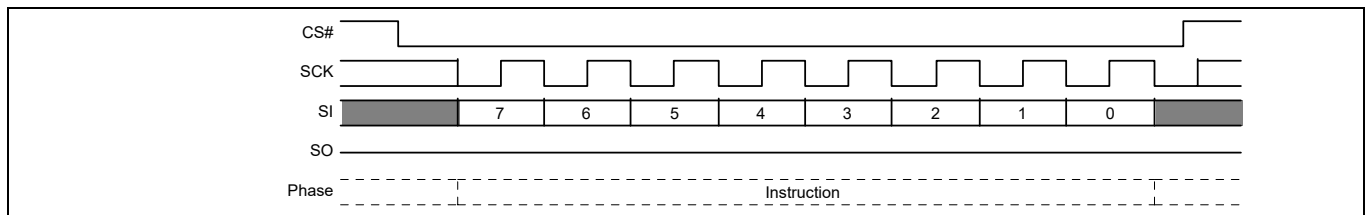
Figure 48 Write Disable (WRDI) command sequence
