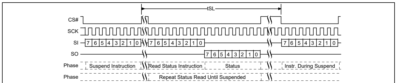
Figure 83 Program or Erase Suspend command sequence
