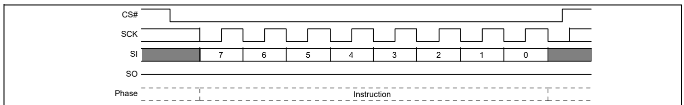
Figure 86 Erase or Program Resume command sequence
