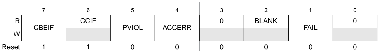
Figure 28-12. Flash Status Register (FSTAT — Normal Mode)
