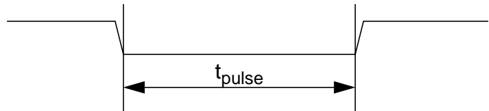
Figure 23-78. Pulse Illustration
