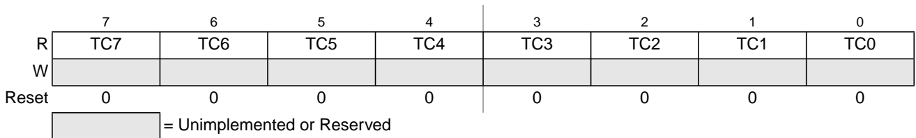
Figure 7-60. Timer Input Capture Holding Register 1 Low (TC1L)
