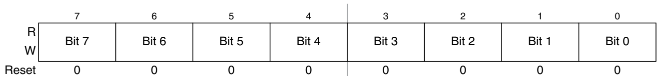
Figure 14-27. Timer Input Capture/Output Compare Register 3 Low (TC3)
