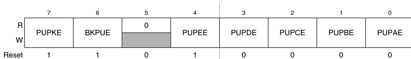
Figure 2-11. S12X_EBI ports, BKGD pin Pull-up Control Register (PUCR)
