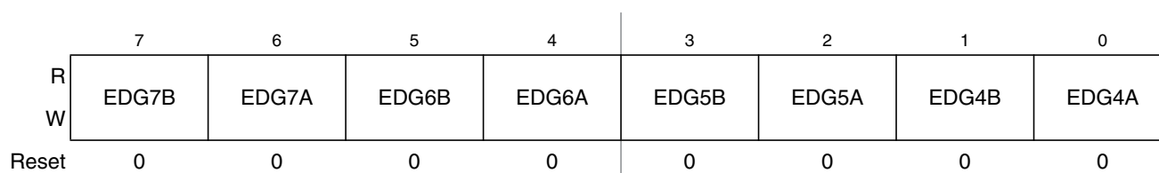
Figure 22-16. Timer Control Register 3 (TCTL3)
