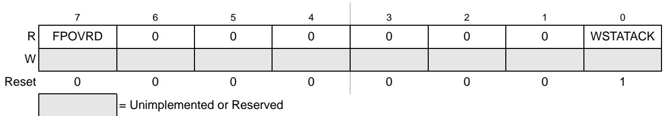
Figure 19-9. Flash Protection Status Register (FPSTAT)
