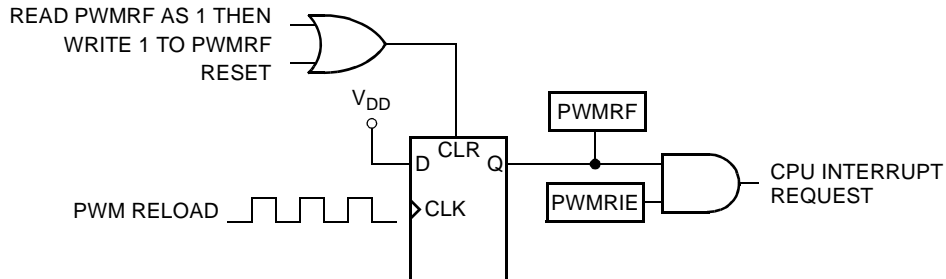
Figure 14-75. PWMRF Reload Interrupt Request
