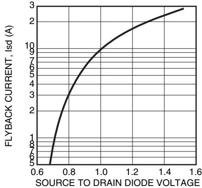
REVERSE DIODE
