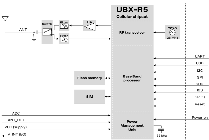
Figure 1: SARA-R500E block diagram
