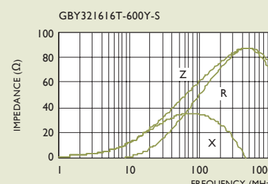
RDC < 0.10Ω Rated Current: 1000mA
