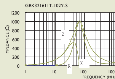
RDC < 0.25Ω Rated Current: 400mA
