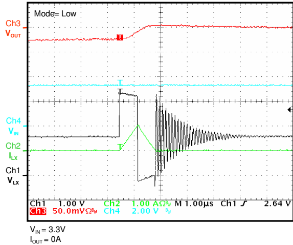
Output Voltage Ripple ( V_{OUT} = 1.5\text{V} ), PSAVE Mode
